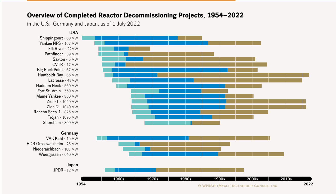
Figure 45 - Overview of Completed Reactor Decommissioning Projects, 1954–2022
